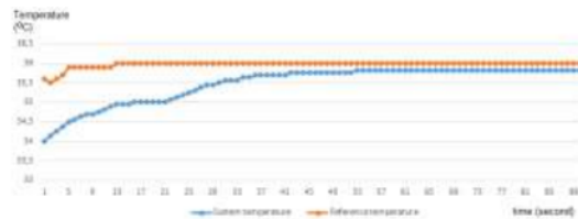
Figure 11. Result of the second experiment for temperature testing process
