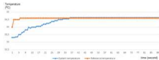
Figure 12. Result of the thirth experiment for temperature testing process
